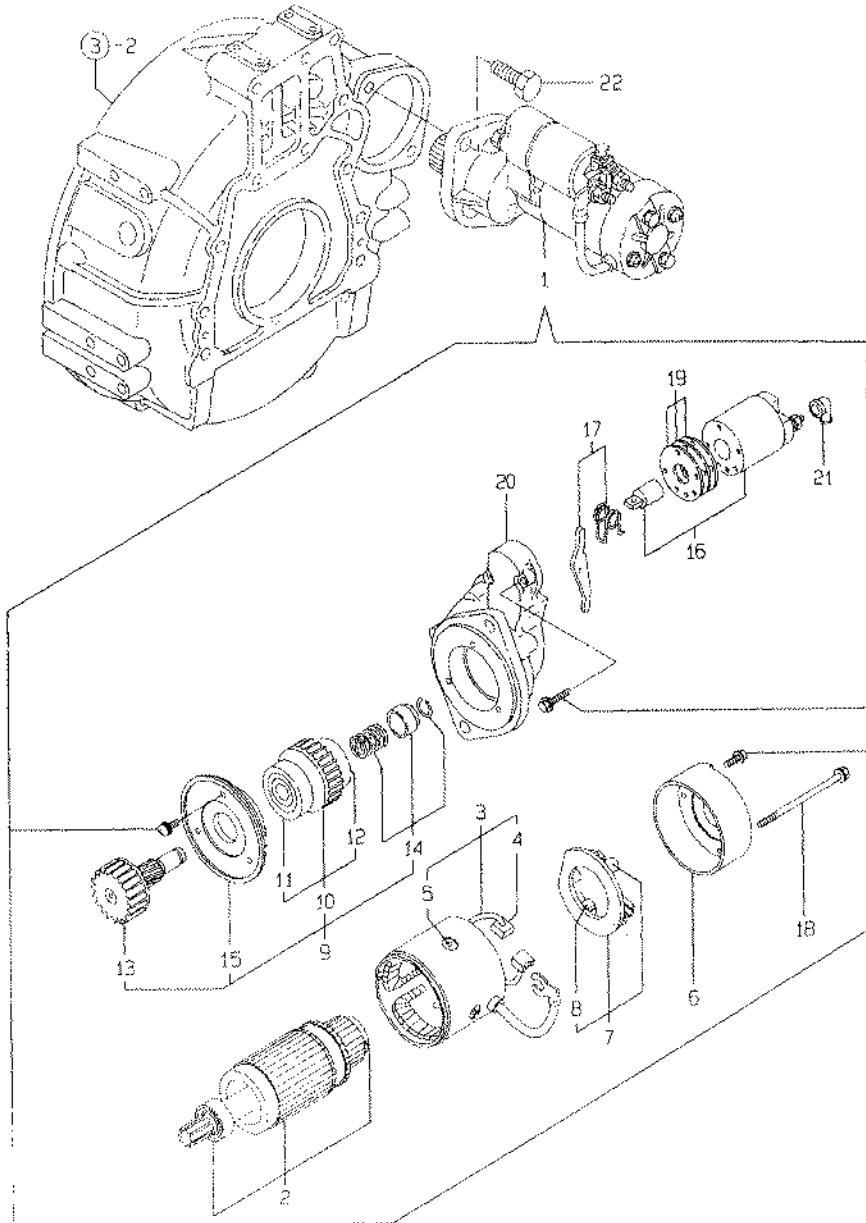
15. STARTING MOTOR
